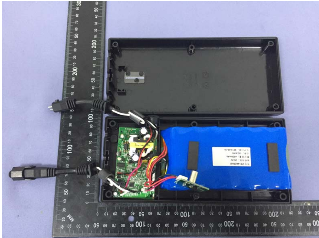
Figure 3 Internal view of battery (内部图)
